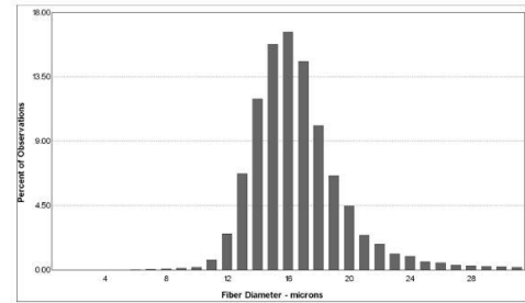
This Test Performed According to I.W.T.O Method 47
